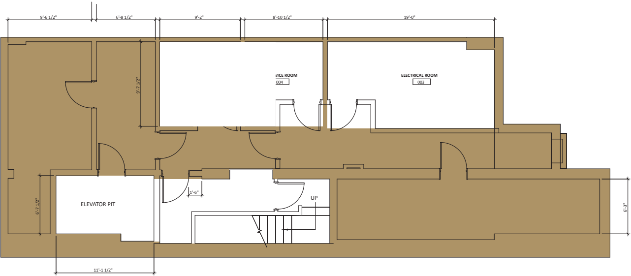
B BASEMENT PLAN SCALE: 1/4" = 1'-0"
